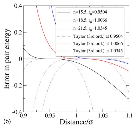
FIG. 2. (Color online) (a) The Lennard-Jones potential v_{LJ}(r) fitted by an effective power-law potential v_{PL}(r) = Ar^{-n} + B covering the most important part of the repulsive part of the potential. The exponent n was chosen to be 18, which optimizes agreement at r_0 = \sigma , where the effective power law exactly matches not just v_{LJ} but also its first two derivatives. Also shown are the Taylor series expansions of v_{LJ}(r) about r=r_m up to third and fourth orders. The RDF g(r)-1 (at T=80 K, p=0 ) is also shown as a convenient reference for thinking about where contributions to potential energy and virial fluctuations come from. (b) Error made in approximating v_{LJ}(r) with different effective power laws matched at different points r_0 and with Taylor expansions up to third order about the same point.
